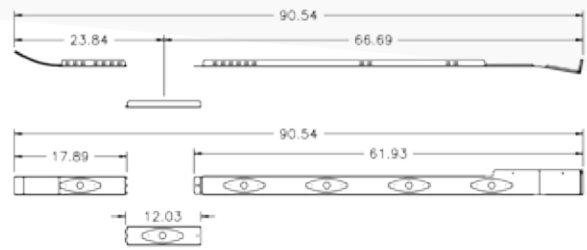
FUEL DOOR LOCATION - DRIVER
